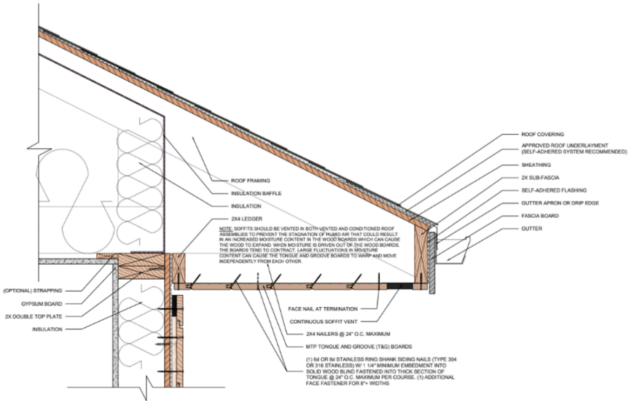
1.0 SOFFIT DETAIL W/ TONGUE AND GROOVE BOARDS
