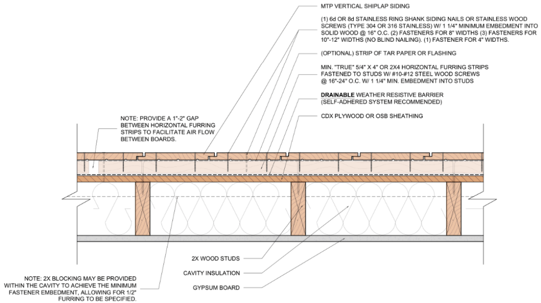
○ MTP VERTICAL SHIPLAP
